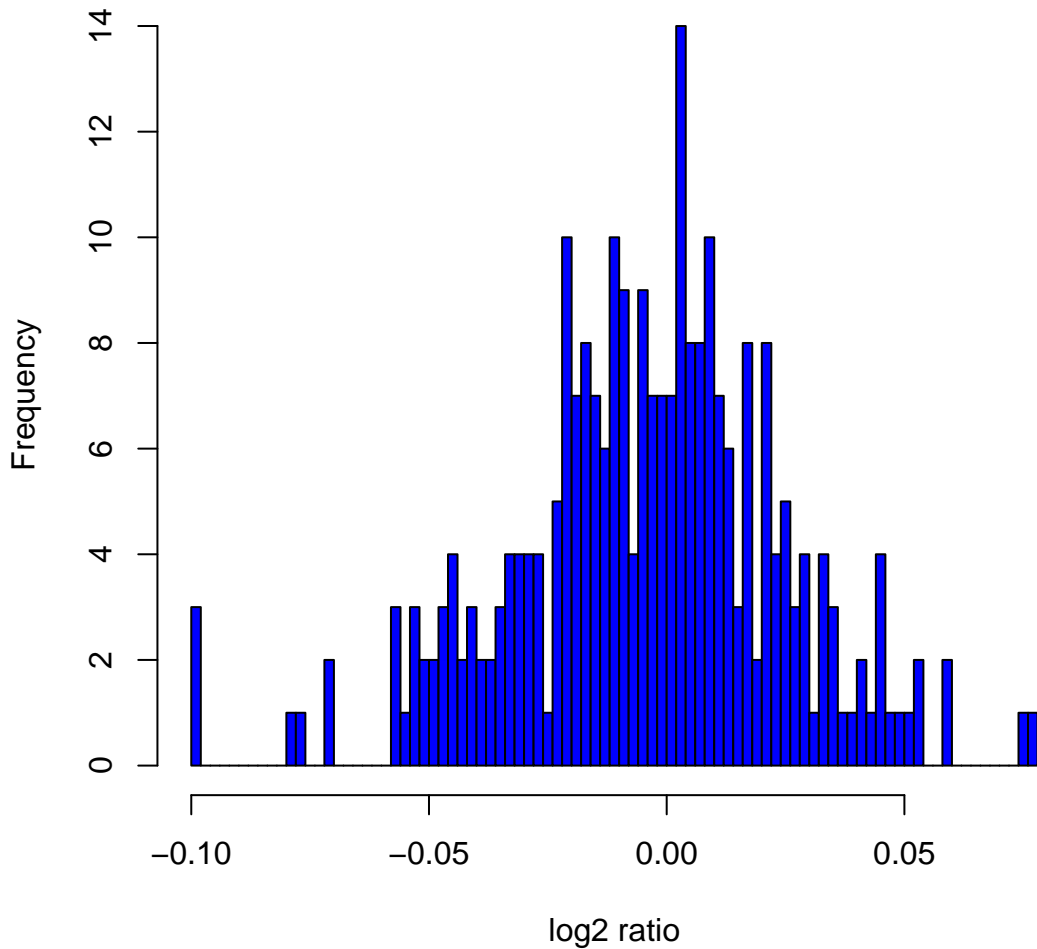
Histogram of \log_2 ratios in 270 HapMap samples at clone Chr9tp-4A6
