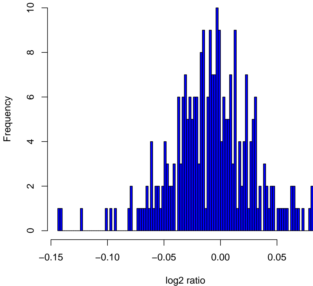
Histogram of log 2 ratios in 270 HapMap samples at clone Chr9tp-4B3
