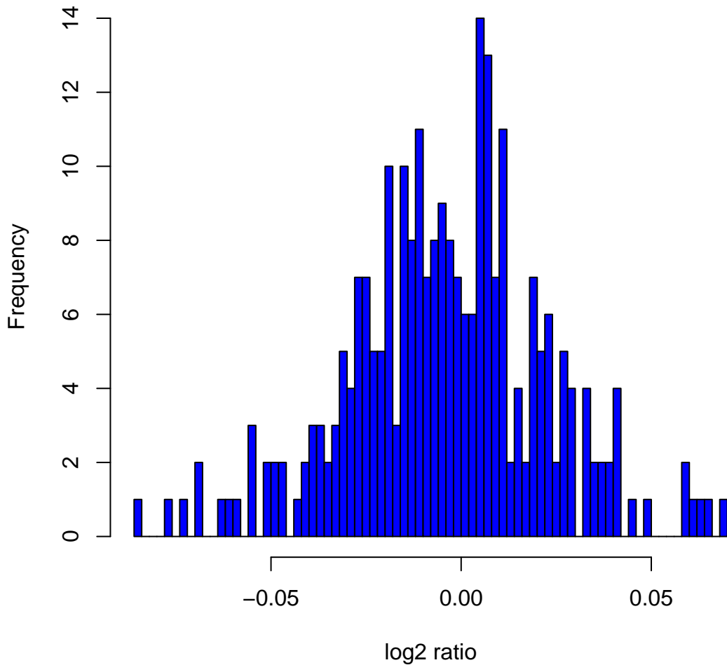
Histogram of log 2 ratios in 270 HapMap samples at clone Chr9tp-4B4
