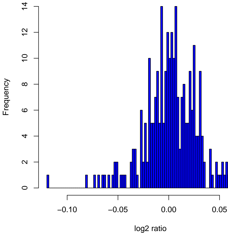
Histogram of log2ratios in 270 HapMap samples at clone Chr9tp-4C2
