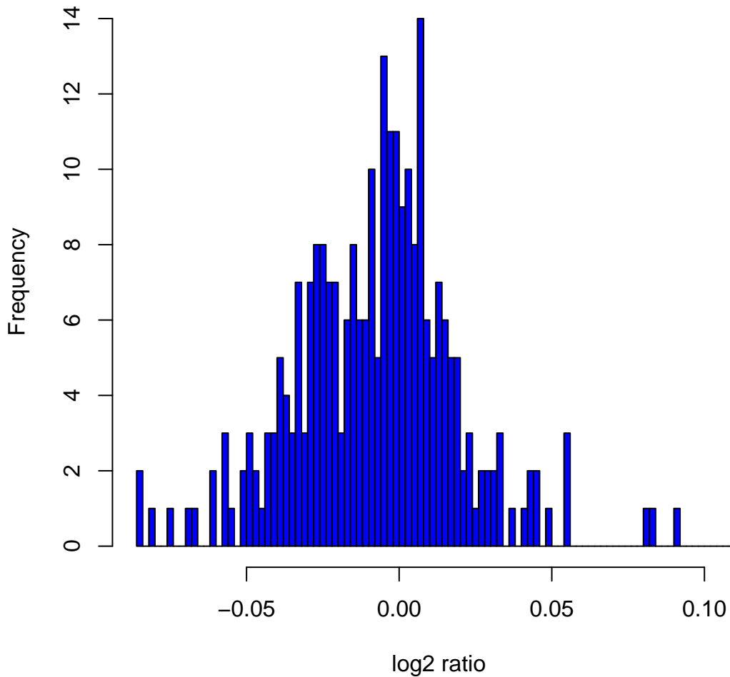
Histogram of log 2 ratios in 270 HapMap samples at clone Chr9tp-4C4
