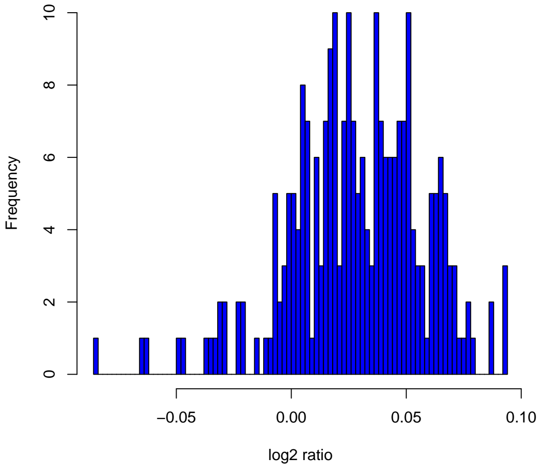
Histogram of \log_2 ratios in 270 HapMap samples at clone Chr9tp-4C5
