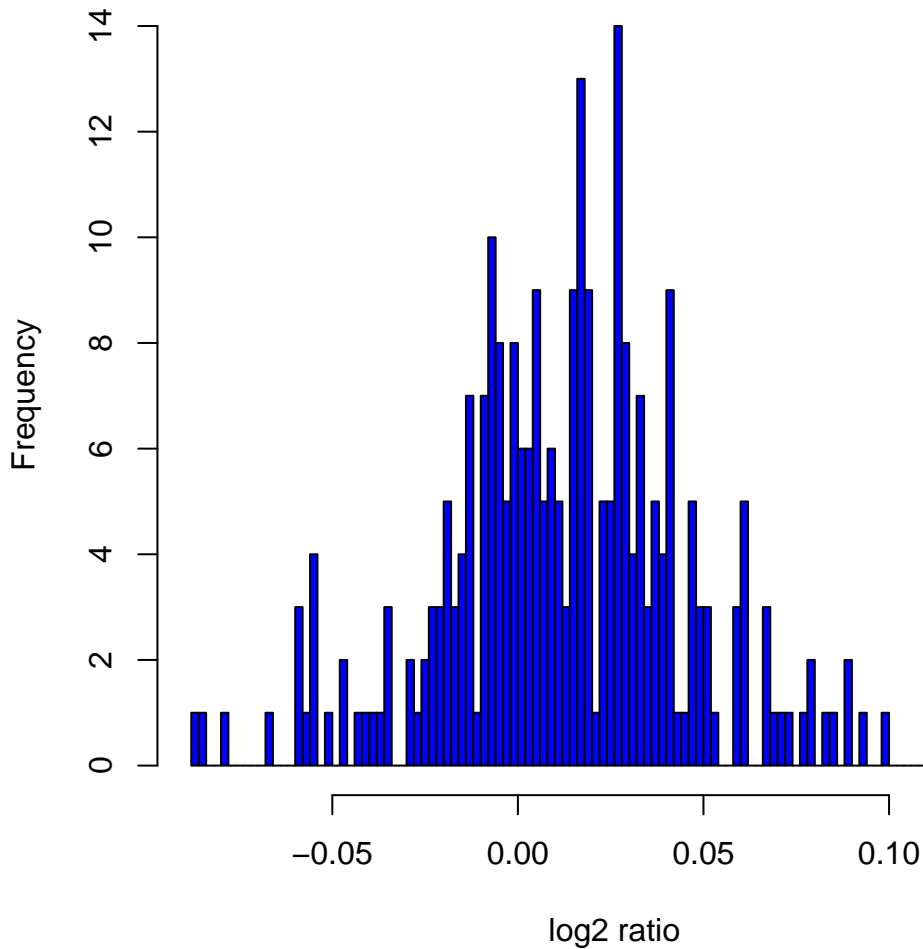
Histogram of log 2 ratios in 270 HapMap samples at clone Chr9tp-4C7
