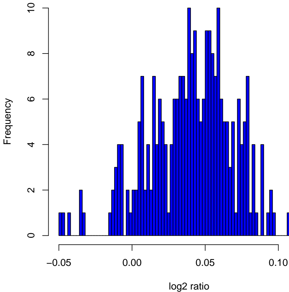
Histogram of log 2 ratios in 270 HapMap samples at clone Chr9tp-4D8
