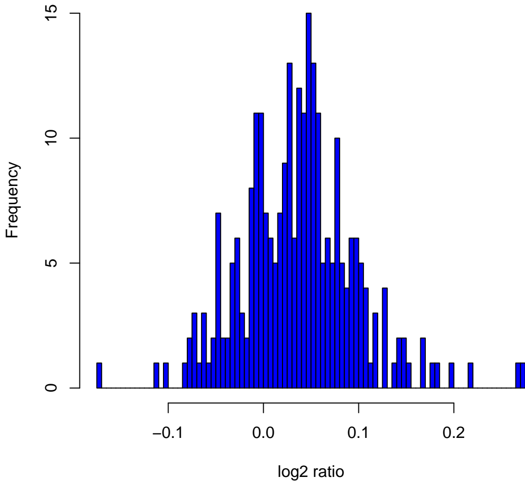
Histogram of log 2 ratios in 270 HapMap samples at clone Chr9tp-4E3
