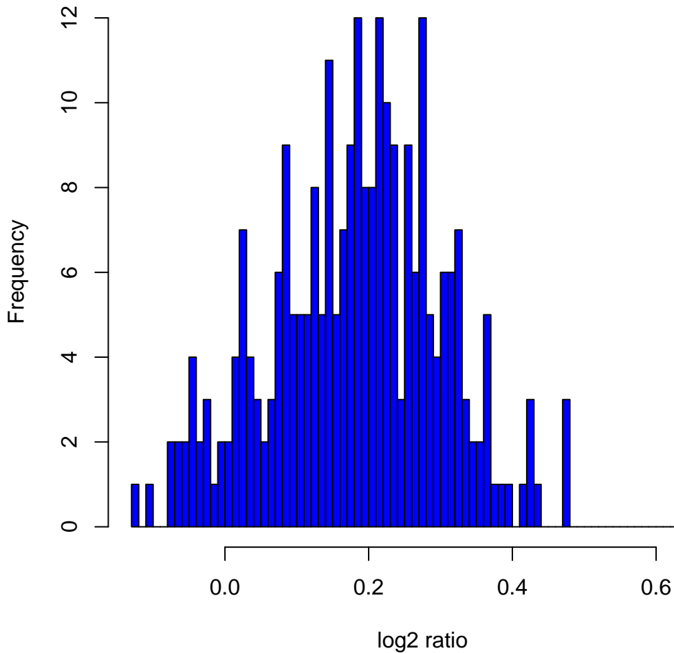
Histogram of log 2 ratios in 270 HapMap samples at clone Chr9tp-4F8
