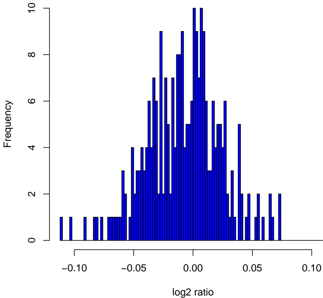
Histogram of log 2 ratios in 270 HapMap samples at clone Chr9tp-4G6
