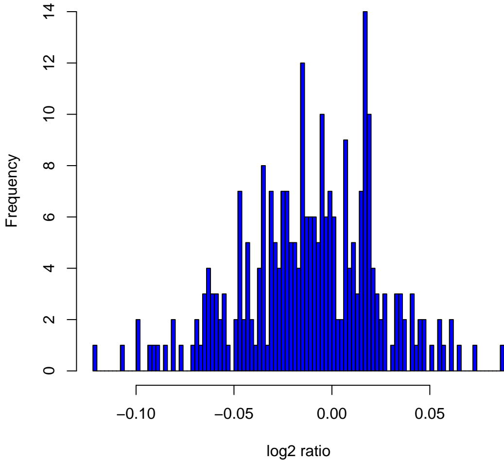
Histogram of log 2 ratios in 270 HapMap samples at clone Chr9tp-4H12
