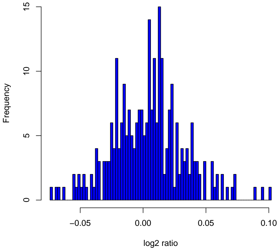
Histogram of log 2 ratios in 270 HapMap samples at clone Chr9tp-4H9
