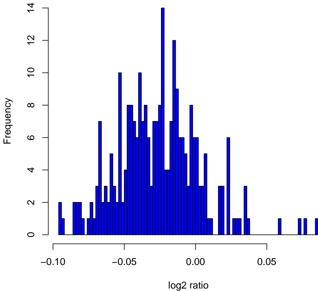
Histogram of log 2 ratios in 270 HapMap samples at clone Chr9tp-5A1
