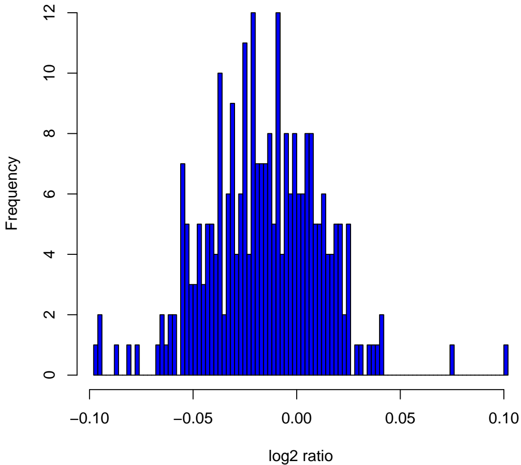
Histogram of \log_2 ratios in 270 HapMap samples at clone Chr9tp-5A5
