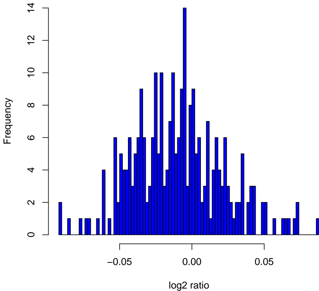
Histogram of \log_2 ratios in 270 HapMap samples at clone Chr9tp-5A9
