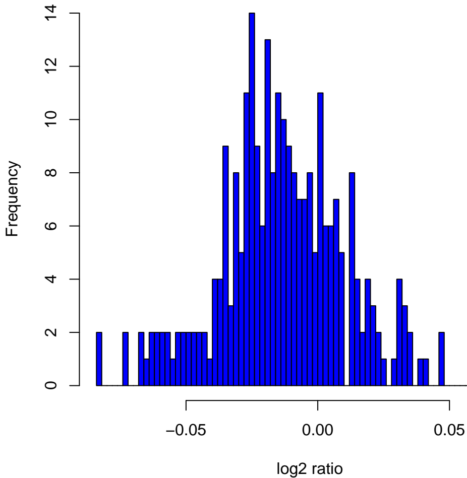
Histogram of log 2 ratios in 270 HapMap samples at clone Chr9tp-5C2
