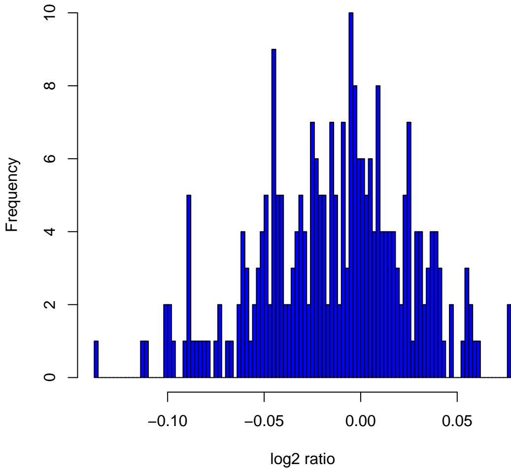
Histogram of \log_2 ratios in 270 HapMap samples at clone Chr9tp-5E8
