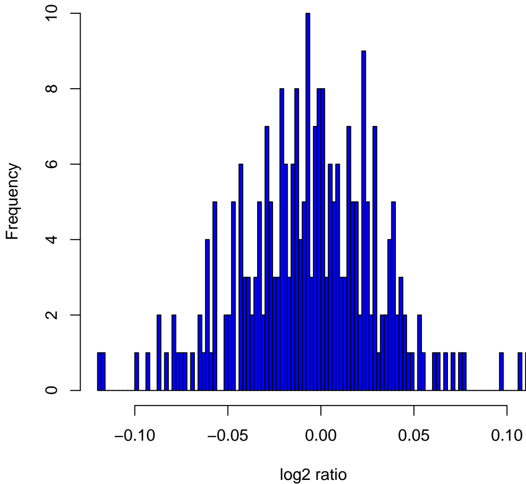
Histogram of log2ratios in 270 HapMap samples at clone Chr9tp-5F8
