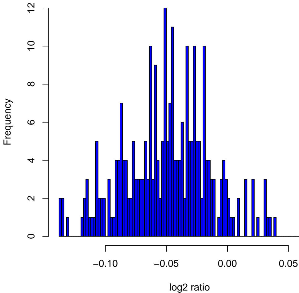
Histogram of log2ratios in 270 HapMap samples at clone Chr9tp-5G12
