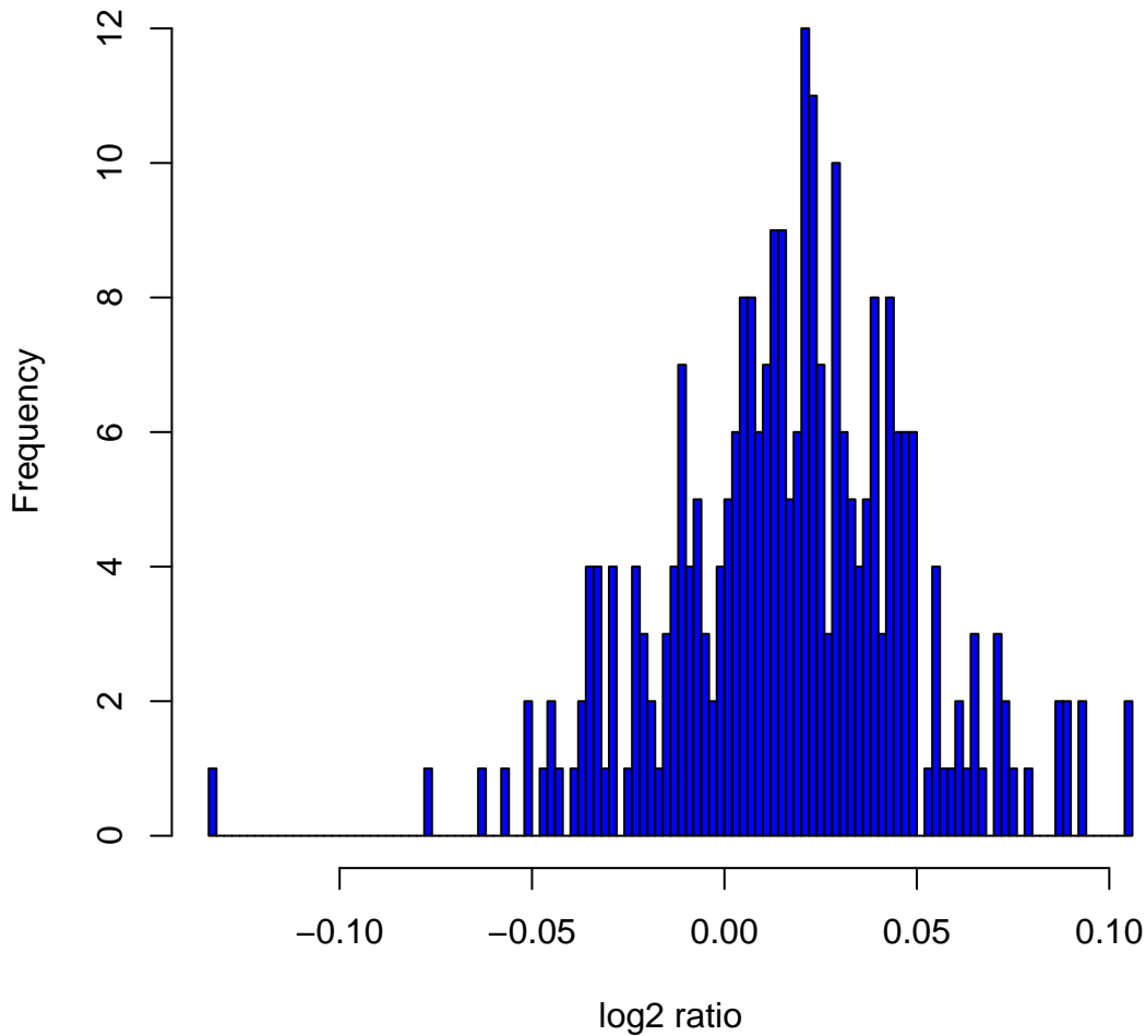
Histogram of \log_2 ratios in 270 HapMap samples at clone Chr9tp-5G6
