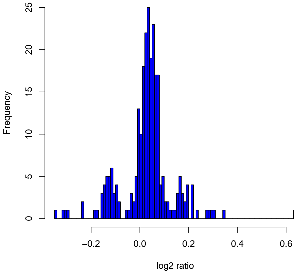
Histogram of log 2 ratios in 270 HapMap samples at clone Chr9tp-5H8
