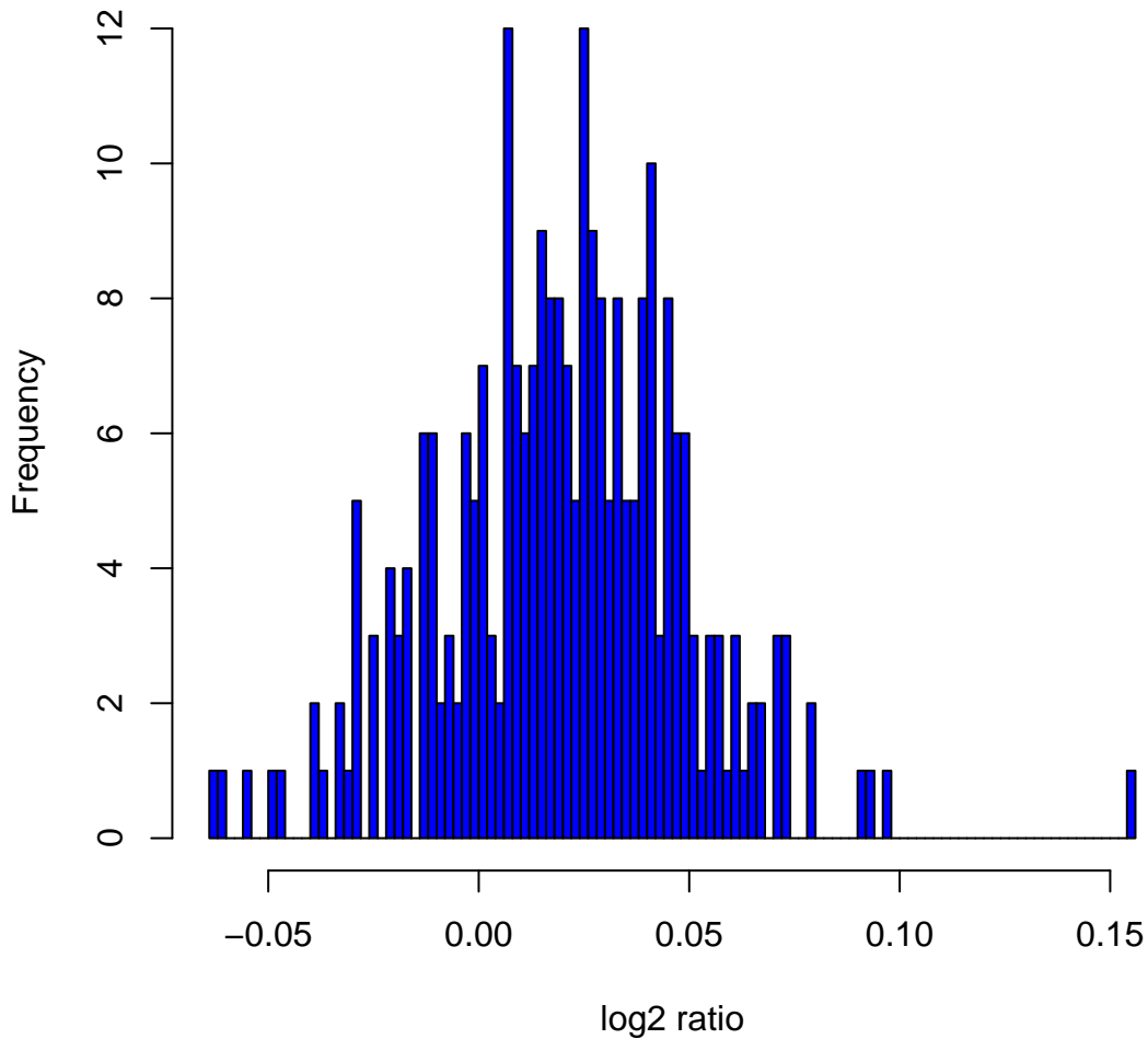
Histogram of log 2 ratios in 270 HapMap samples at clone Chr9tp-5H9
