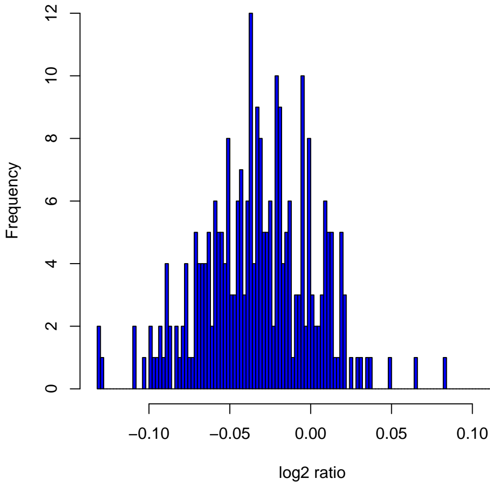
Histogram of log 2 ratios in 270 HapMap samples at clone Chr9tp-6A11
