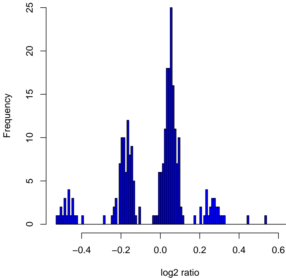
Histogram of log 2 ratios in 270 HapMap samples at clone Chr9tp-6A2
