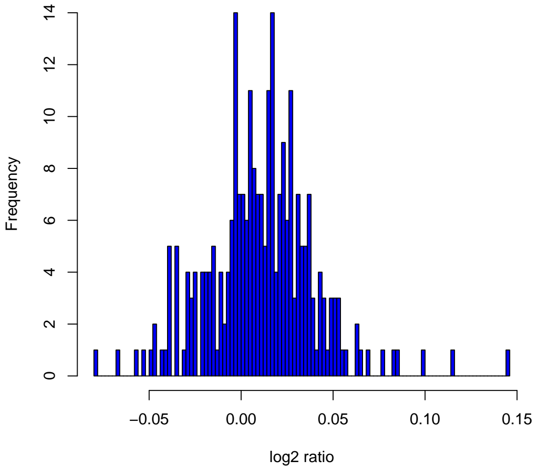
Histogram of \log_2 ratios in 270 HapMap samples at clone Chr9tp-6B9
