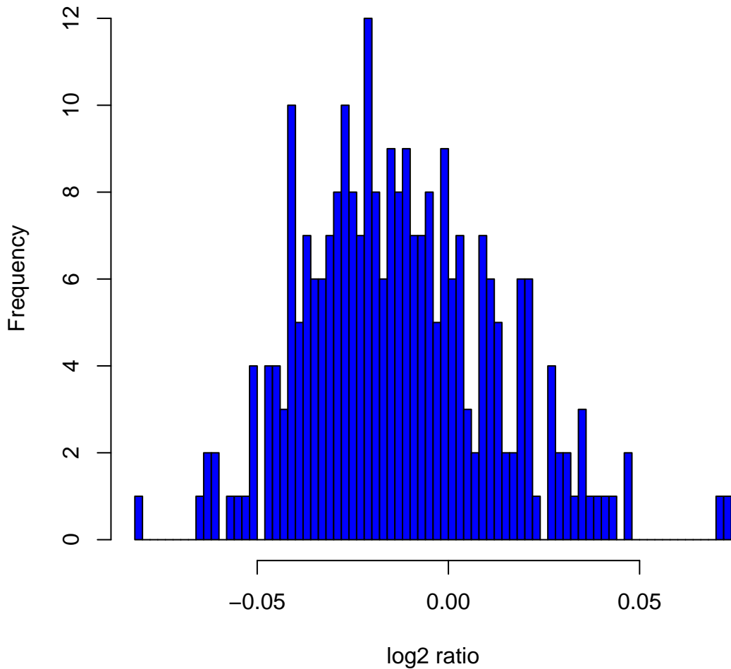
Histogram of log 2 ratios in 270 HapMap samples at clone Chr9tp-6C4
