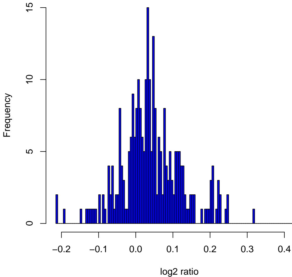
Histogram of \log_2 ratios in 270 HapMap samples at clone Chr9tp-6E7
