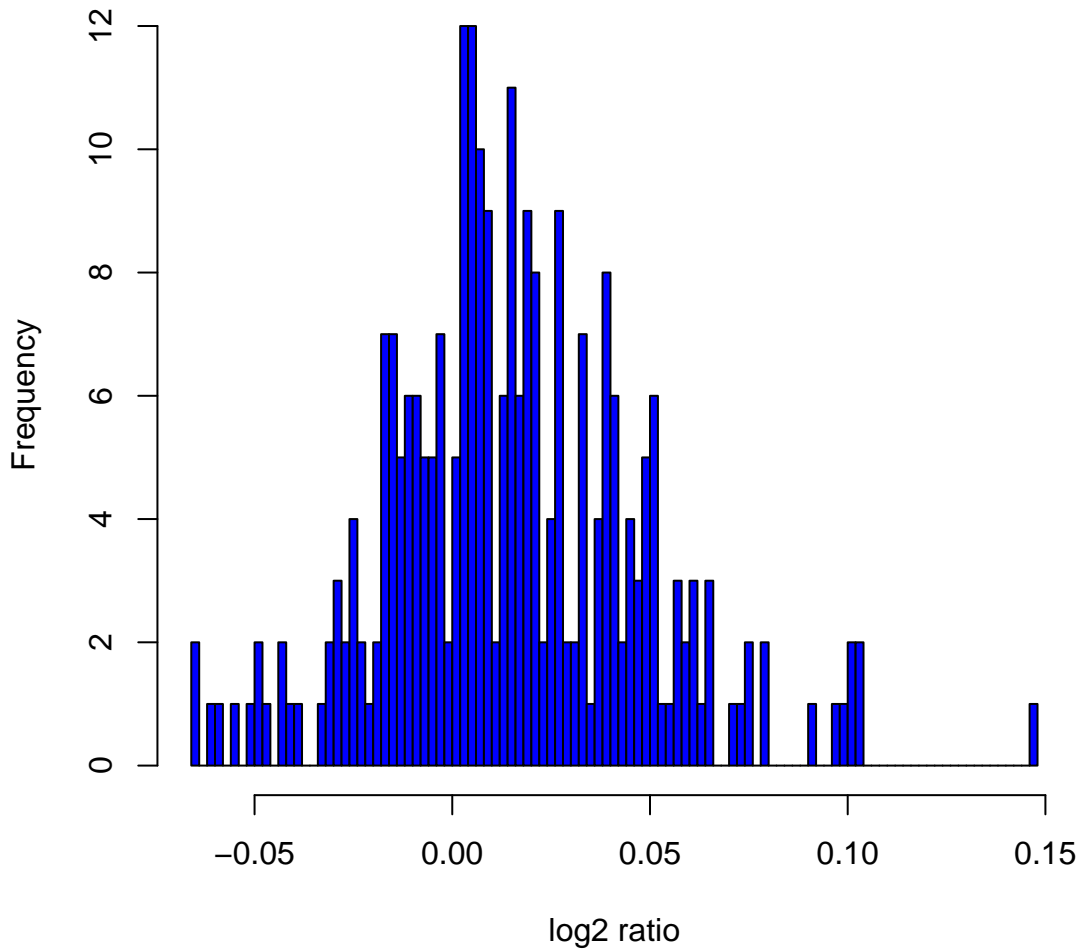
Histogram of log2ratios in 270 HapMap samples at clone Chr9tp-6F4
