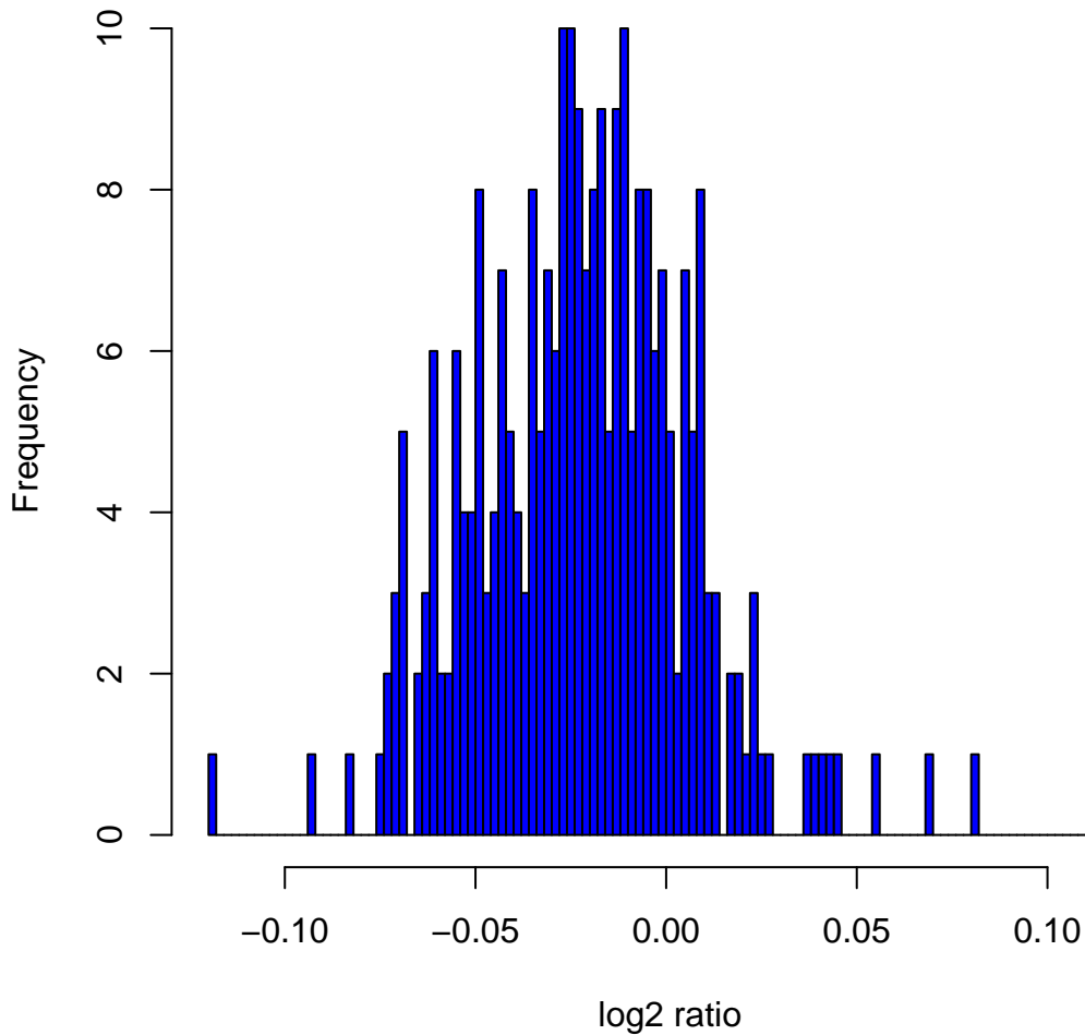
Histogram of log 2 ratios in 270 HapMap samples at clone Chr9tp-6G11
