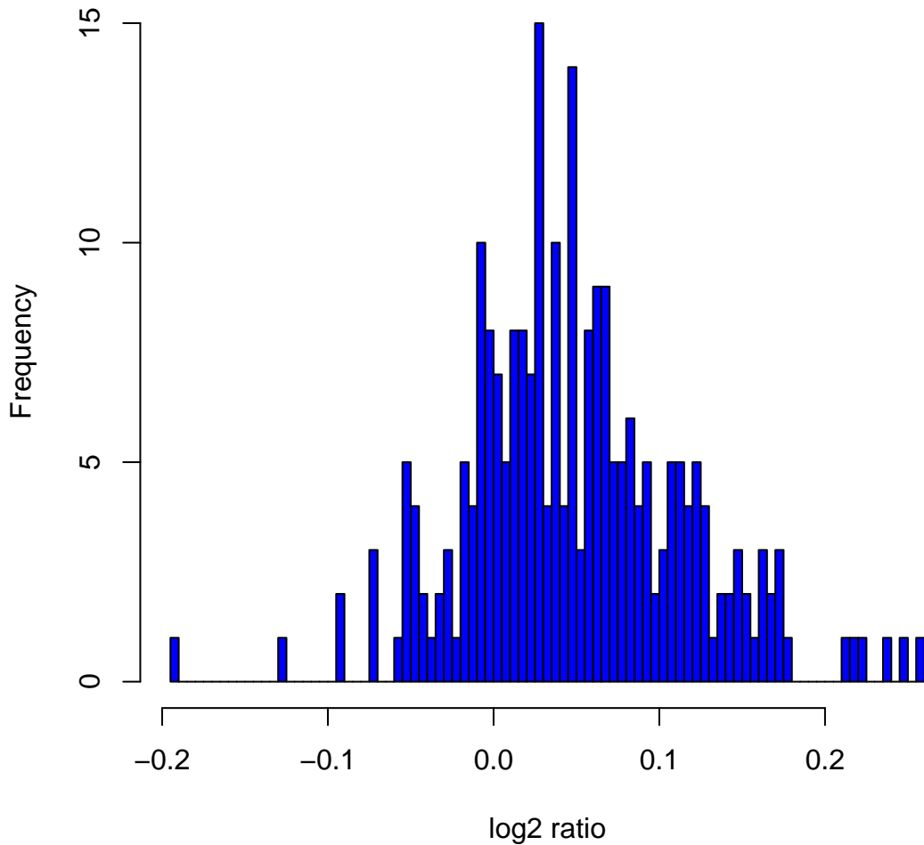
Histogram of log 2 ratios in 270 HapMap samples at clone Chr9tp-7A8
