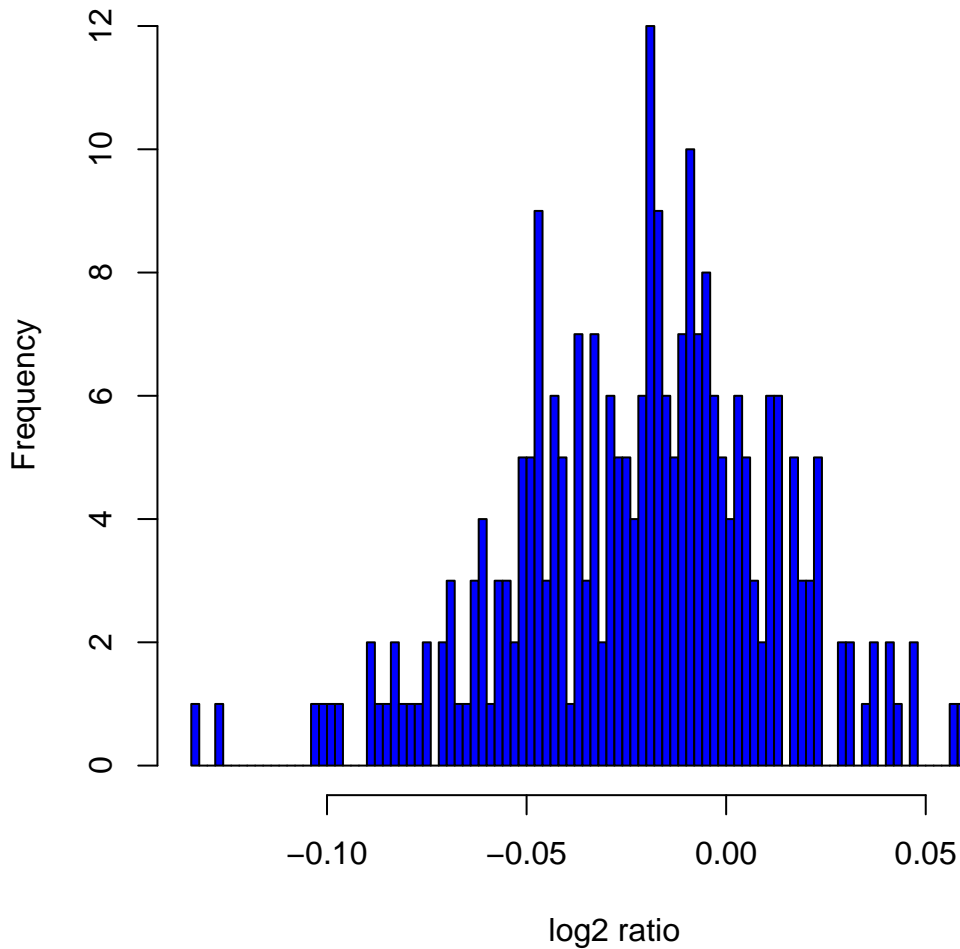
Histogram of \log_2 ratios in 270 HapMap samples at clone Chr9tp-7C5
