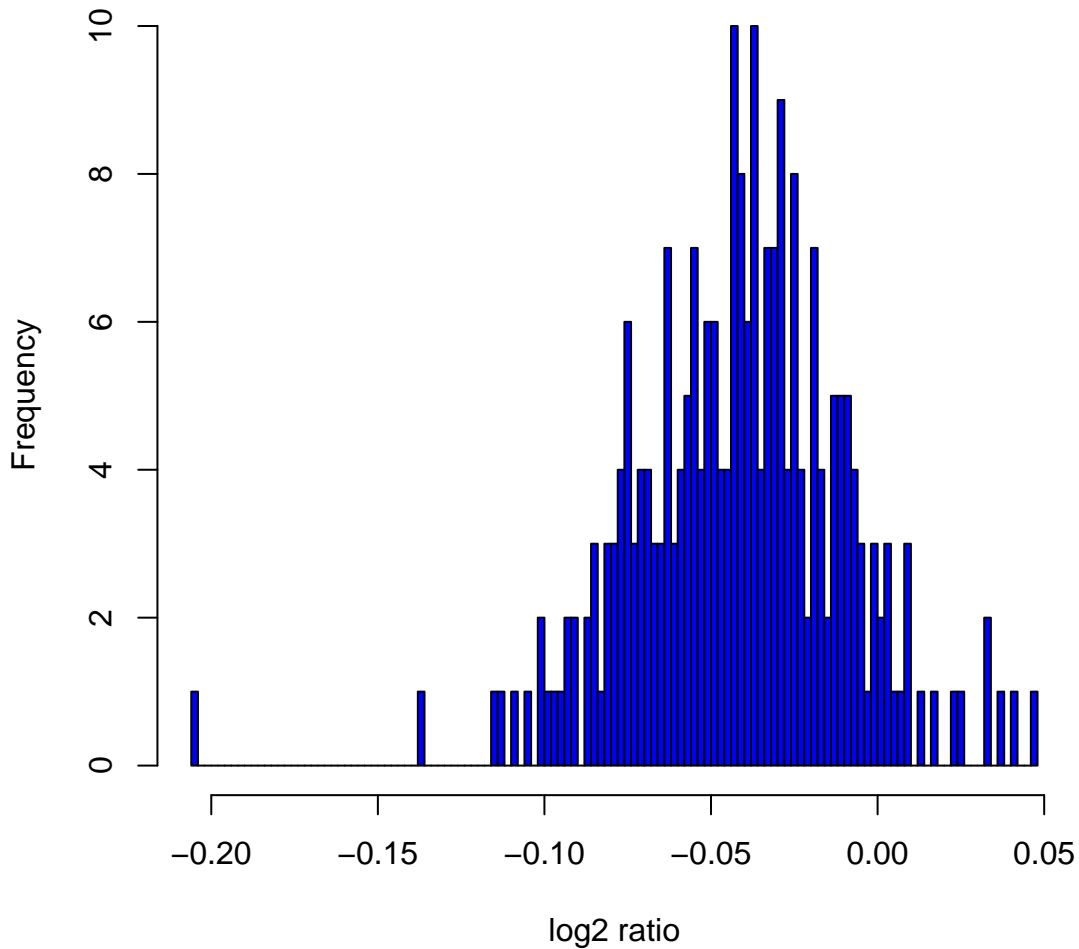
Histogram of log 2 ratios in 270 HapMap samples at clone Chr9tp-7D9
