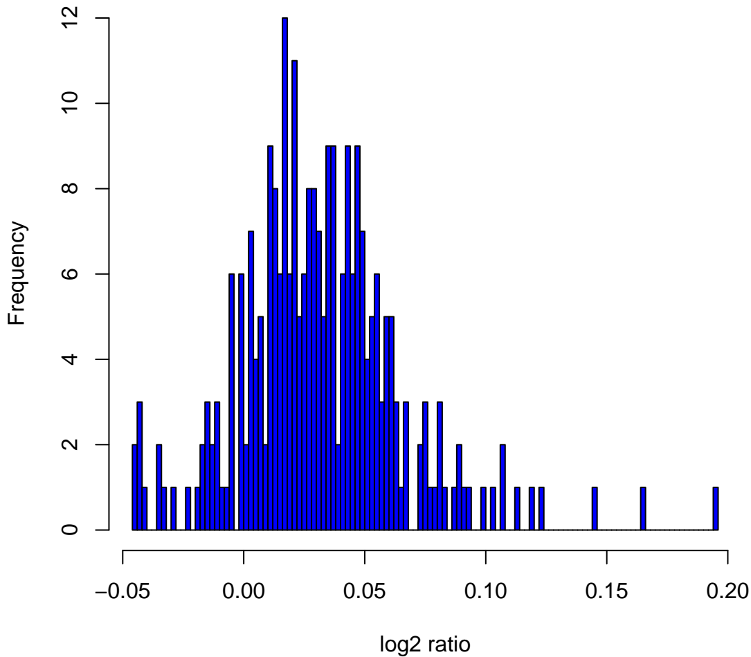
Histogram of log2ratios in 270 HapMap samples at clone Chr9tp-7F6
