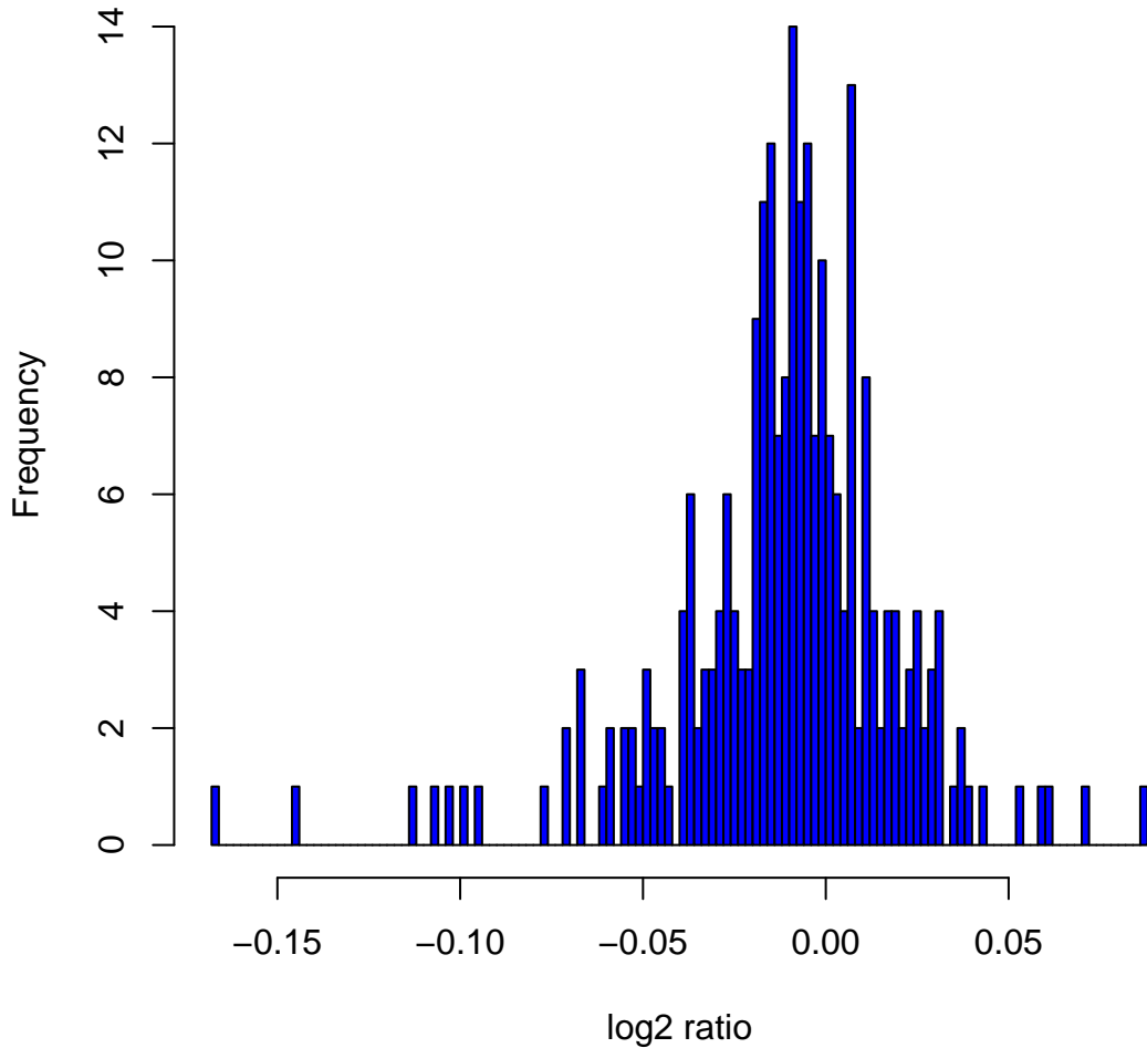
Histogram of log2ratios in 270 HapMap samples at clone Chr9tp-7F7
