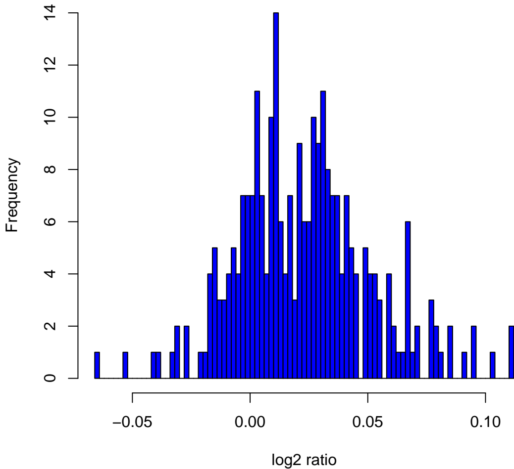
Histogram of log 2 ratios in 270 HapMap samples at clone Chr9tp-8A1
