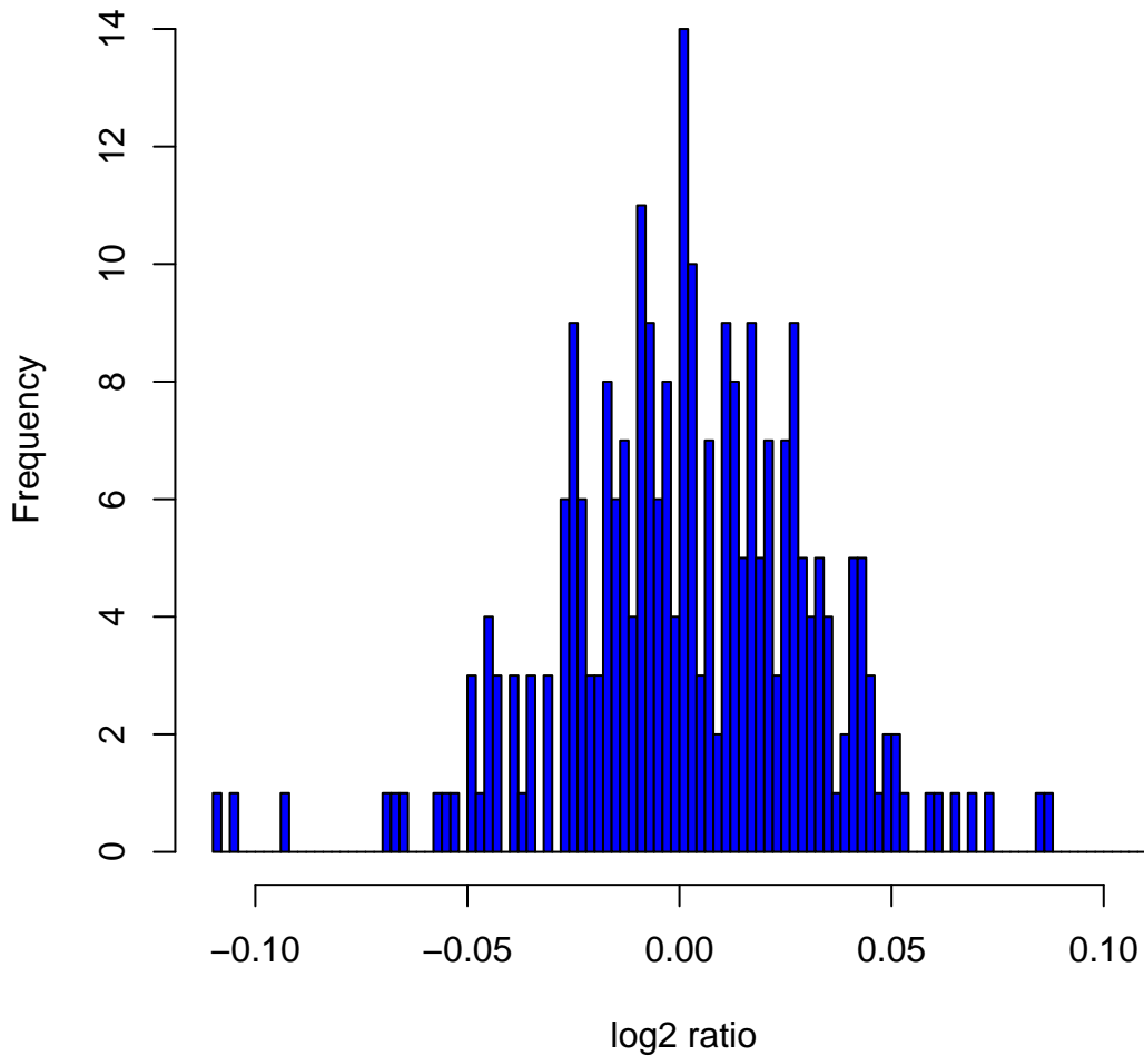
Histogram of log 2 ratios in 270 HapMap samples at clone Chr9tp-8A2
