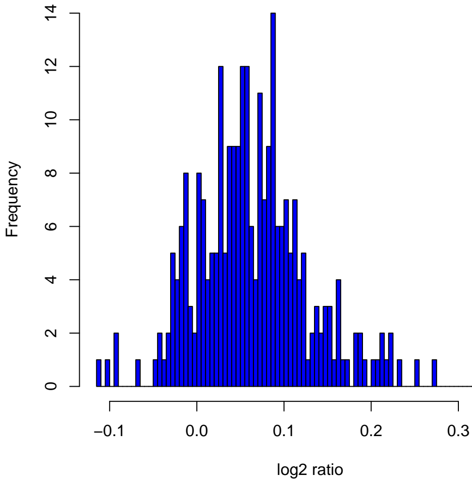
Histogram of log 2 ratios in 270 HapMap samples at clone Chr9tp-8A6
