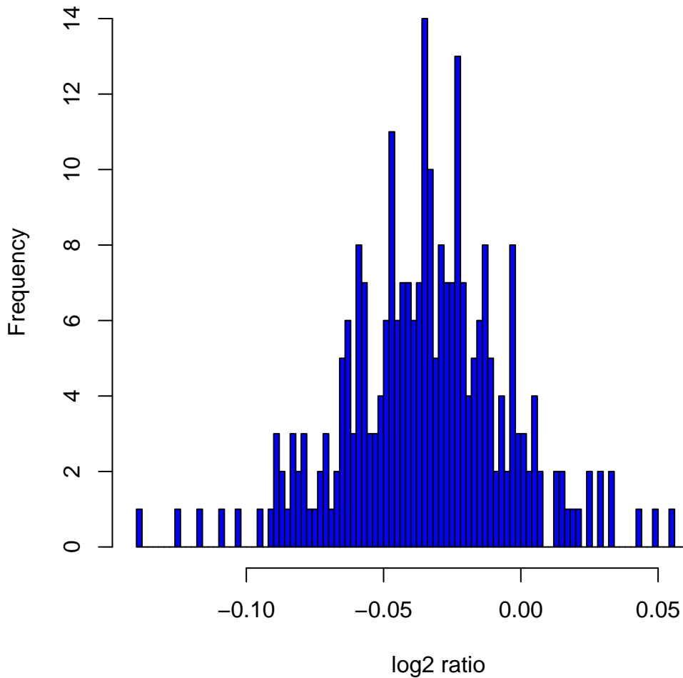
Histogram of log 2 ratios in 270 HapMap samples at clone Chr9tp-8D5
