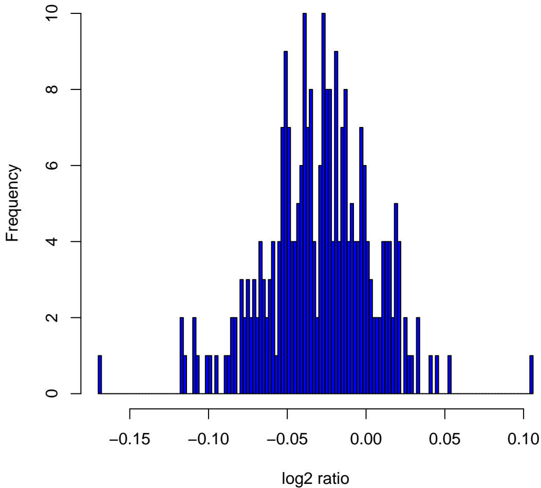
Histogram of log 2 ratios in 270 HapMap samples at clone Chr9tp-8D7
