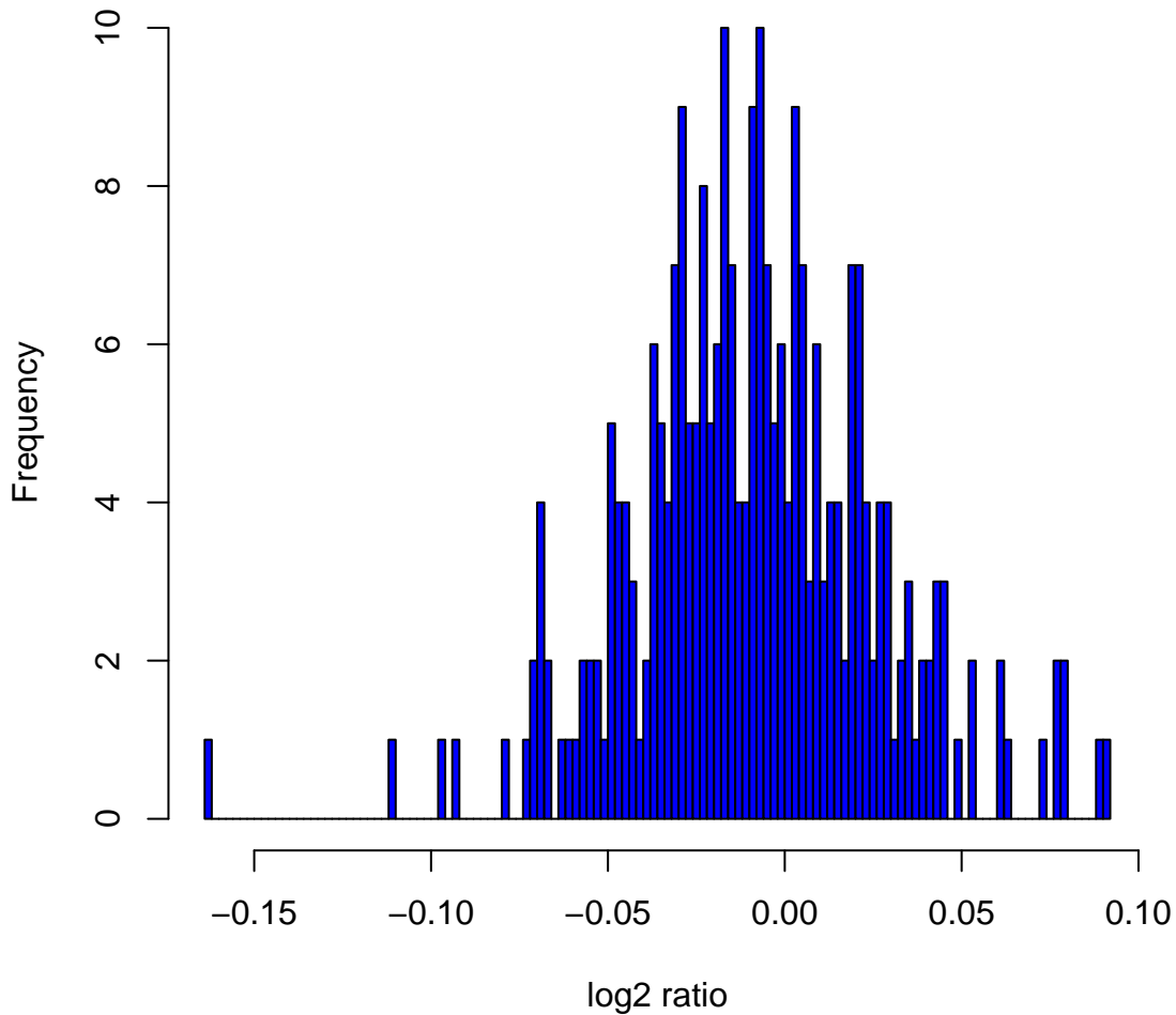
Histogram of log2ratios in 270 HapMap samples at clone Chr9tp-8E9
