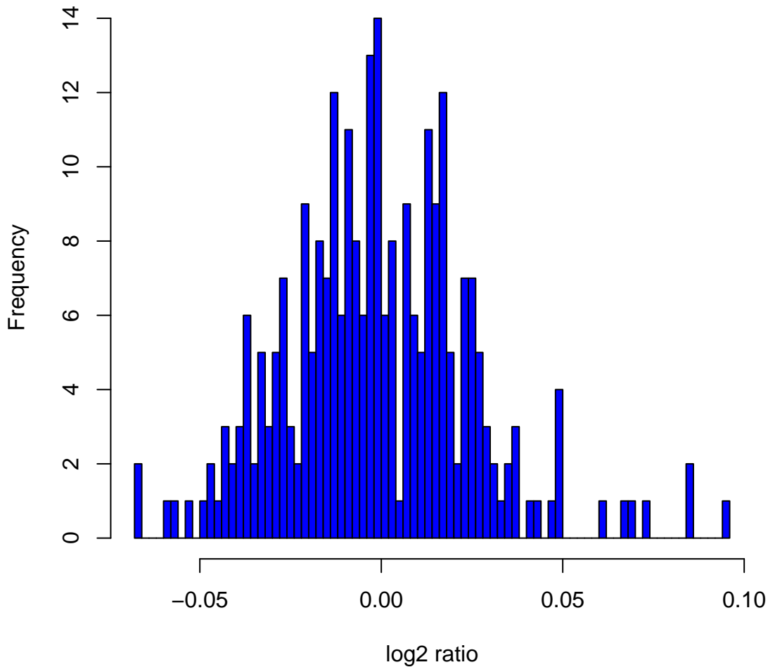
Histogram of log2ratios in 270 HapMap samples at clone Chr9tp-8F1
