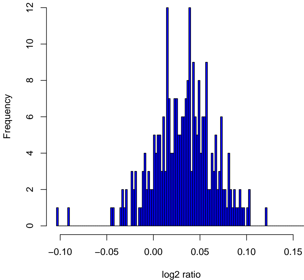
Histogram of log2ratios in 270 HapMap samples at clone Chr9tp-8F6
