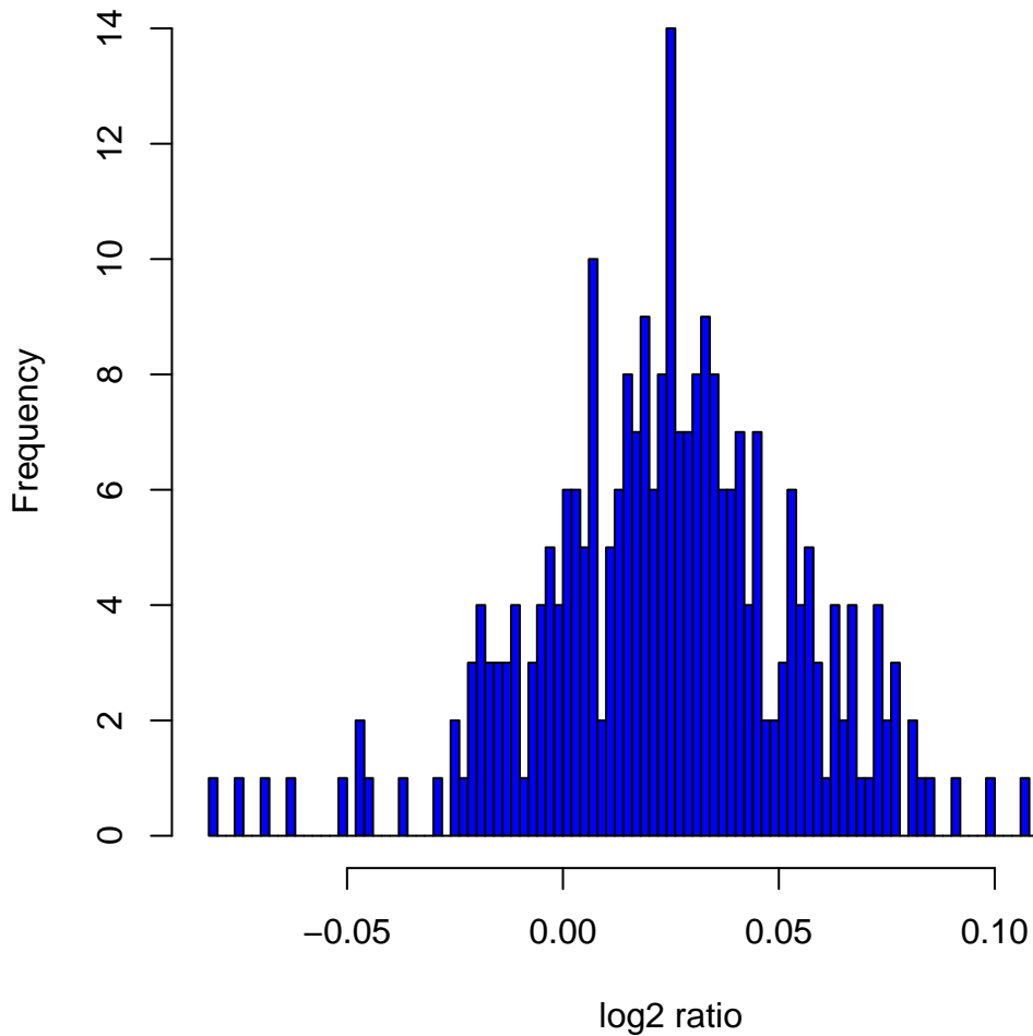
Histogram of log2ratios in 270 HapMap samples at clone Chr9tp-8F7
