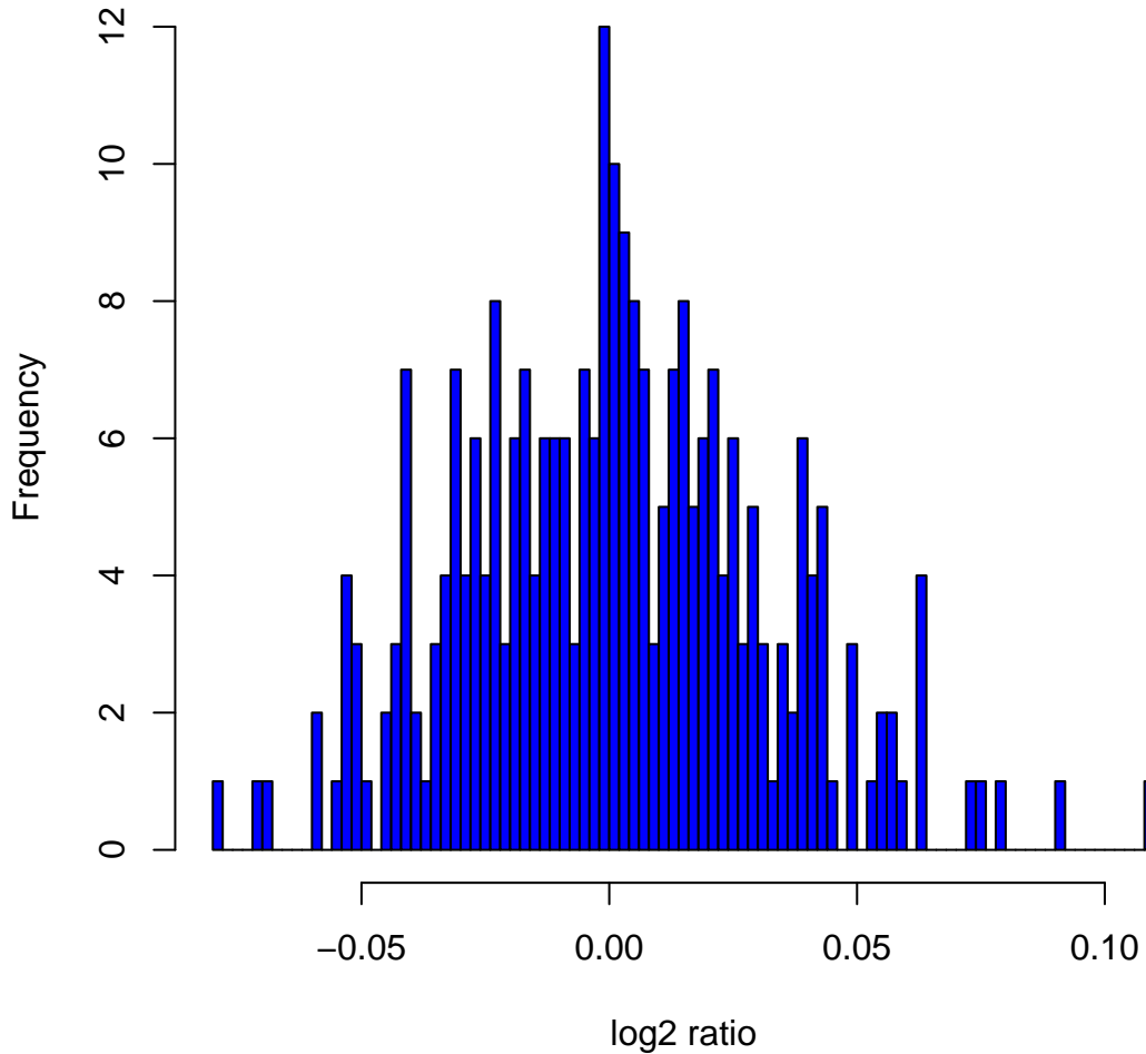
Histogram of log 2 ratios in 270 HapMap samples at clone Chr9tp-8H12
