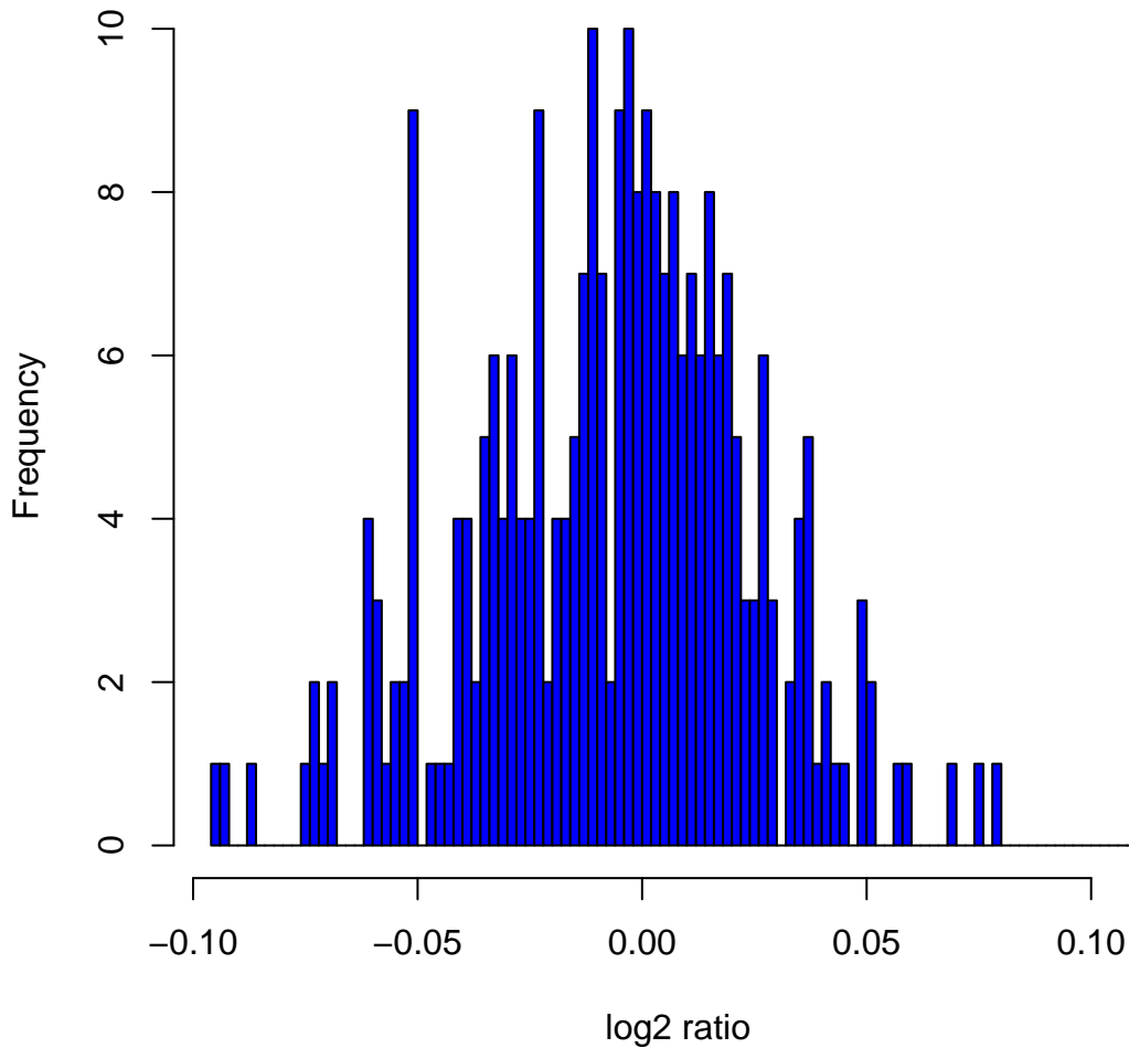
Histogram of log 2 ratios in 270 HapMap samples at clone Chr9tp-9A1
