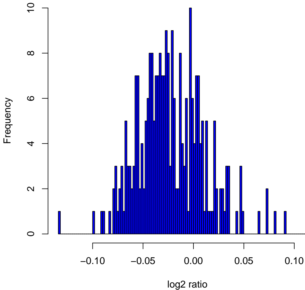
Histogram of \log_2 ratios in 270 HapMap samples at clone Chr9tp-9A3
