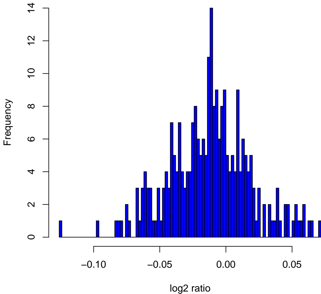
Histogram of \log_2 ratios in 270 HapMap samples at clone Chr9tp-9B5
