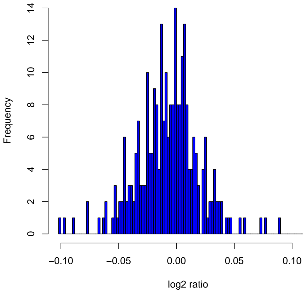
Histogram of log2ratios in 270 HapMap samples at clone Chr9tp-9B6
