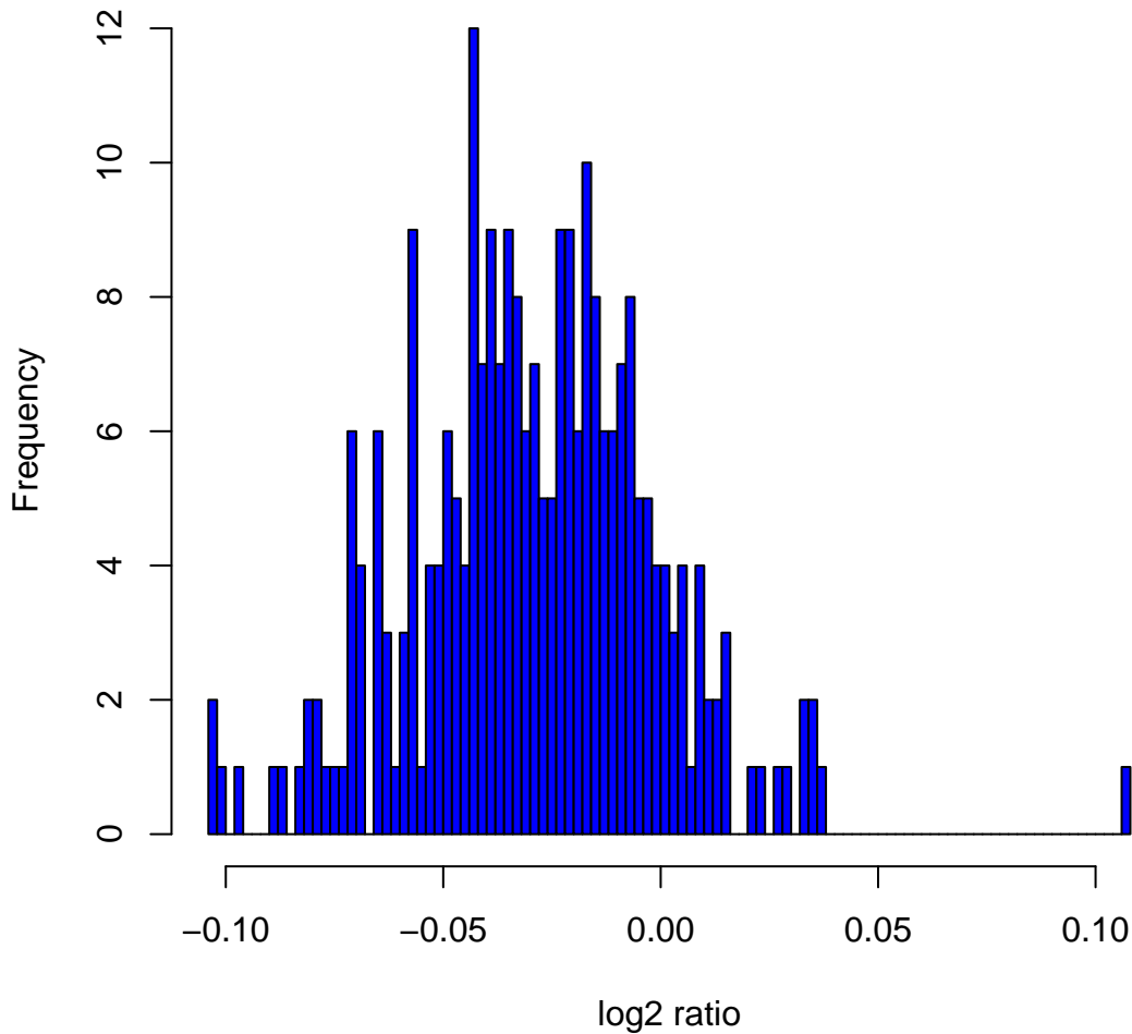
Histogram of log 2 ratios in 270 HapMap samples at clone Chr9tp-9C5
